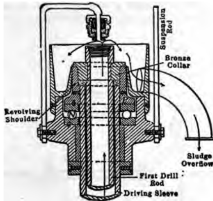
Fig. 70. Swivel Head for Drilling Machine.
